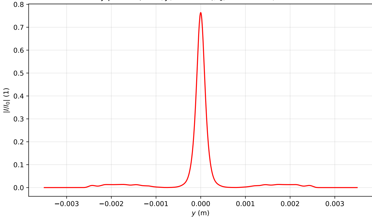
Intensity profile I(x=0, y, z=1.911)/I_0 , \text{Pin}=9.0\text{Pcr} , artificial time
